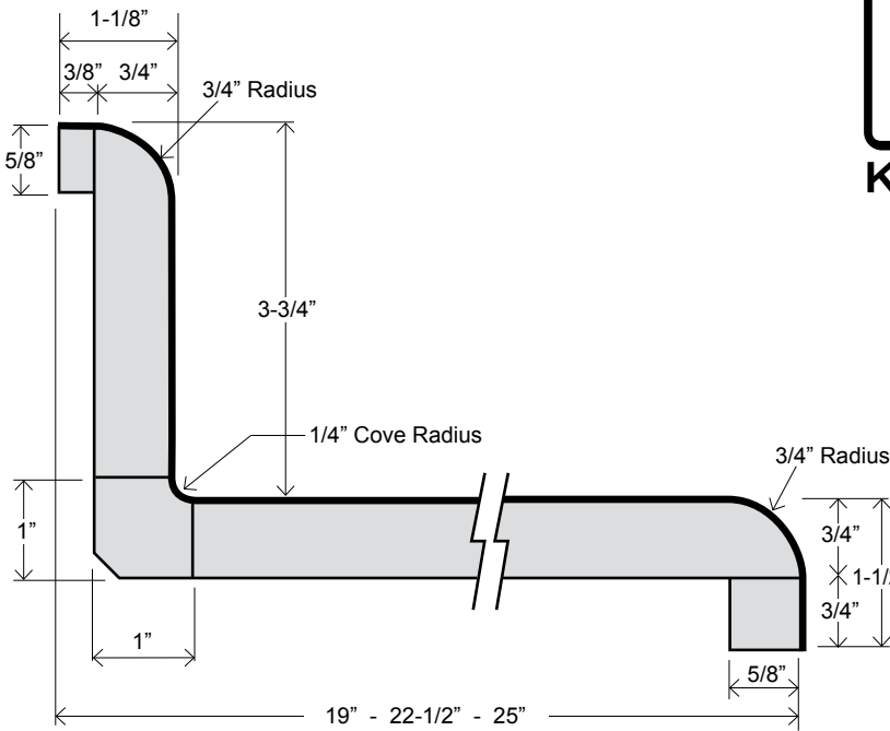
KITCHEN & VANITY TOP PTV 19 PTV 22-1/2 PTK 25
