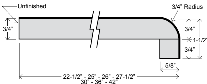
FLAT DECK TOP PTF 22-1/2 PTF 25 PTF 26 PTF 27-1/2 PTF 30 PTF 36 PTF 42
